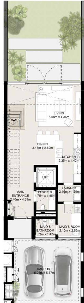
Ground Floor
